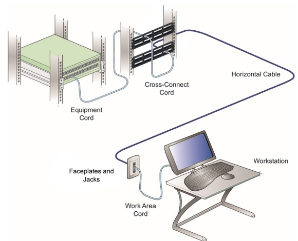
Figure 1. Typical horizontal channel design
