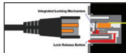
Inside View of Locking Mechanism
