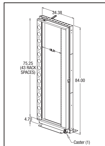
XSW Front View
