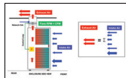
AEHC Single Enclosure Diagram (Side View)
